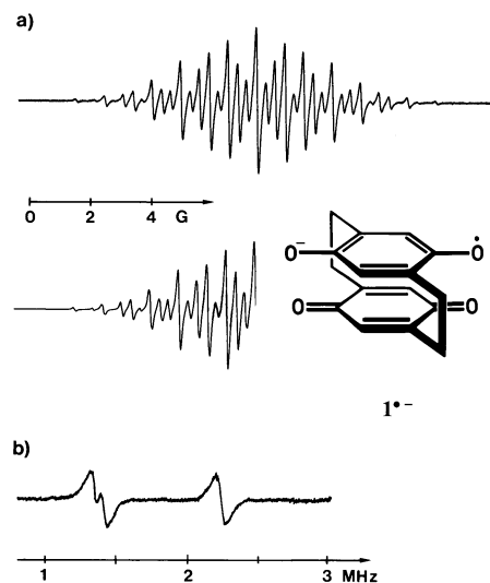
Figure 2. (a) ESR spectrum of the radical anion 1^{\bullet-} in DME/kryptofix ® 222 at 220 K together with a simulation using the data in Table 2; (b) ^1\text{H} special triple resonance spectrum of 1^{\bullet-} in DME/kryptofix ® 222 at 220 K
