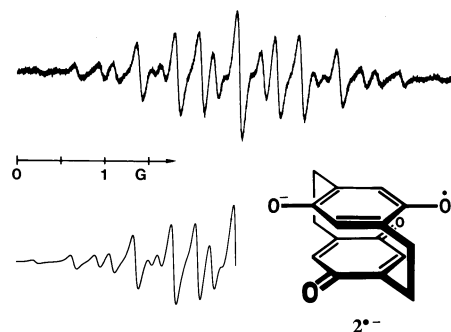
Figure 3. ESR spectrum of the radical anion 2^{\bullet-} in DME/kryptofix ® 222 at 220 K together with a simulation using the data in Table 2
