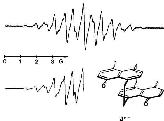
Figure 5. ESR spectrum of the radical anion 4^{\bullet-} in DME/kryptofix ® 222 at 220 K together with a simulation using the data in Table 2
