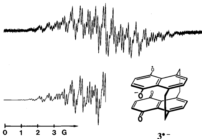
Figure 4. ESR spectrum of the radical anion 3^{\bullet-} in DME/kryptofix ® 222 at 300 K together with a simulation using the data in Table 2
