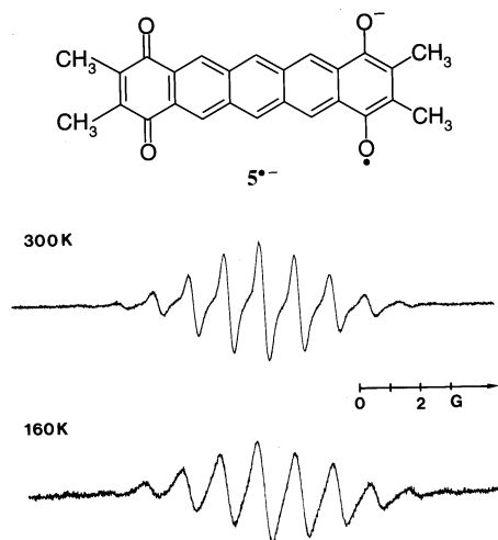
Figure 6. ESR spectra of the radical anion 5^{\bullet-} in MTHF/kryptofix ® 222 at 300 and at 160 K
