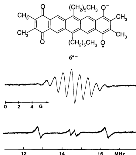
Figure 7. ESR spectrum of the radical anion 6^{\bullet-} in MTHF/kryptofix ® 222 at 200 K and ^1\text{H} -ENDOR spectrum of 6^{\bullet-} in DME/kryptofix ® 222 at 220 K
