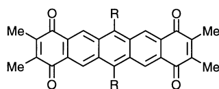
5: R = H 6: R = hexyl
